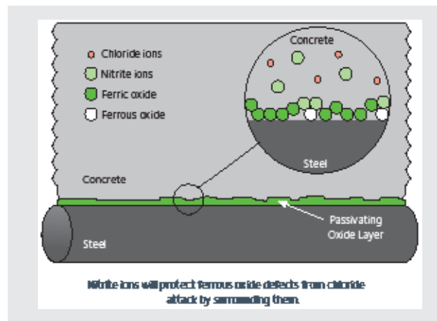
Figure 3C - Calcium Nitrite Protect of Steel
