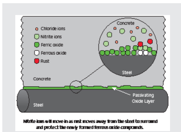
Figure 3D - Calcium Nitrite Protect of Steel
