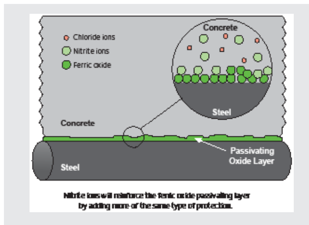
Figure 3B - Calcium Nitrite Protect of Steel
