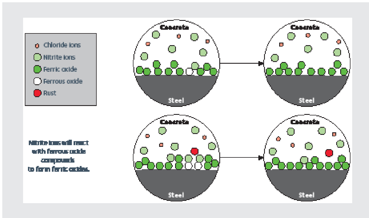
Figure 3 - Calcium Nitrite Protection of Steel
