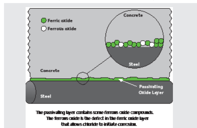
Figure 1 - Naturally Occurring Protective Oxide Layer
