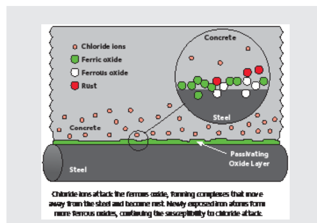
Figure 2 - Chloride Ion Attack of Steel
